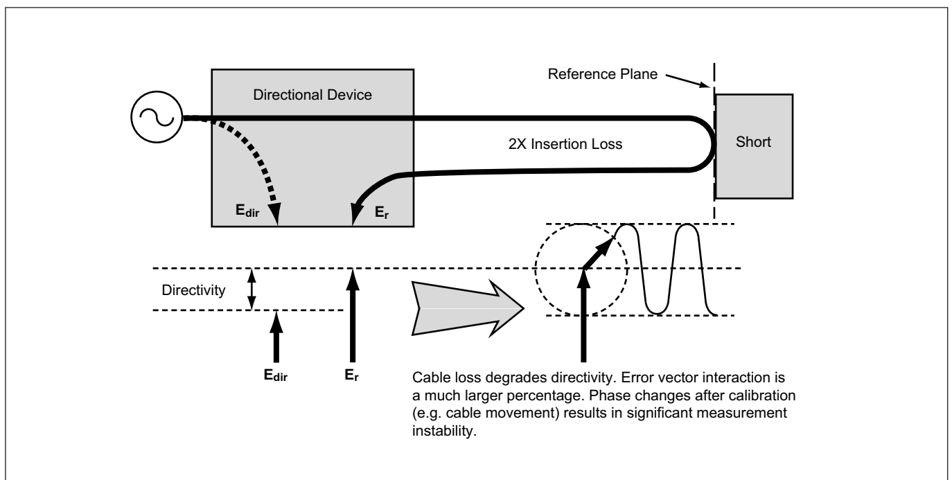
Figure 5. Moving test port away from the directional device decreases calibration stability
