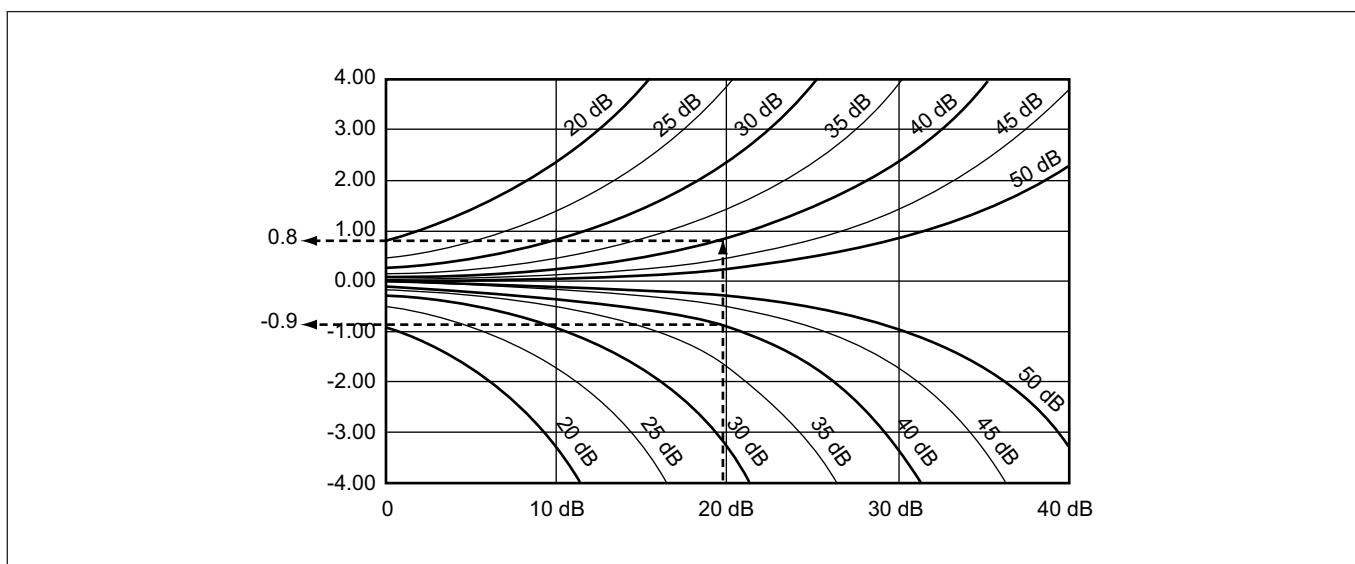
Figure 4. Return Loss Uncertainty Chart. 20 dB Return Loss measured with 40 dB directivity = -0.9 dB worst case measurement uncertainty.
