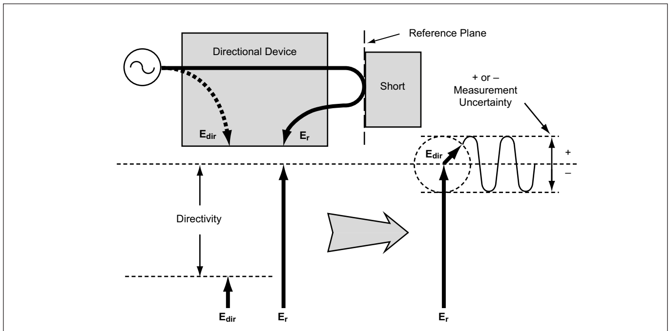
Figure 3. Measurement uncertainty as a result of directivity signal interaction.
