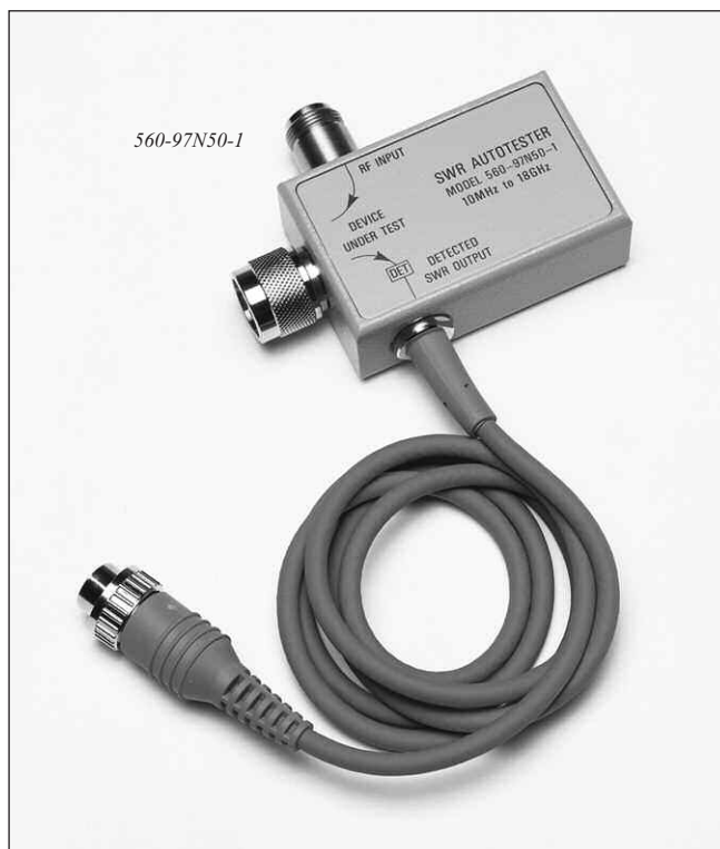
Figure 1. Anritsu Autotesters
